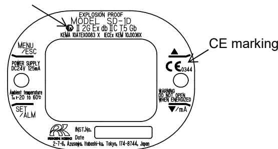
ATEX/IECEx, CE marking type name plate
