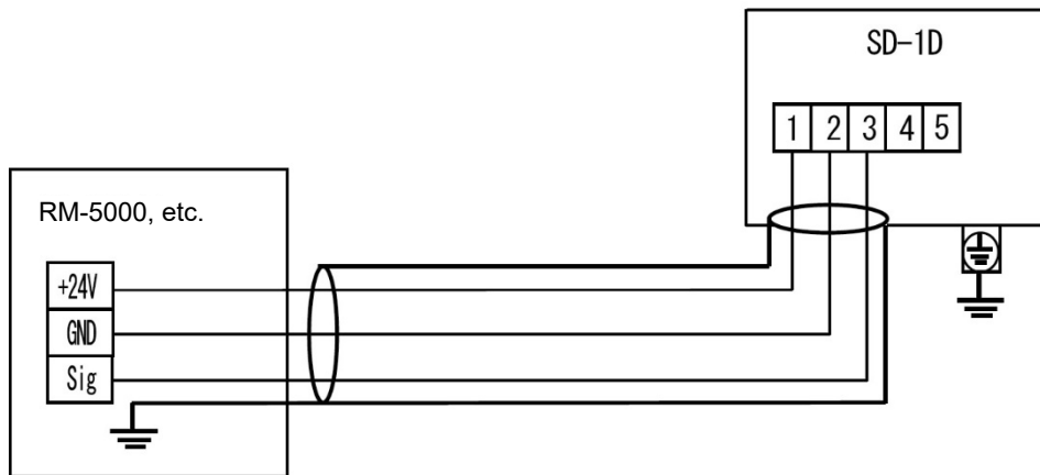
Connecting to the upper unit (DCS, PLC)
