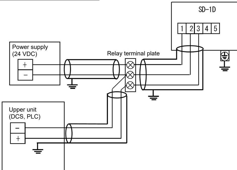
Connecting to the upper unit (DCS, PLC)
