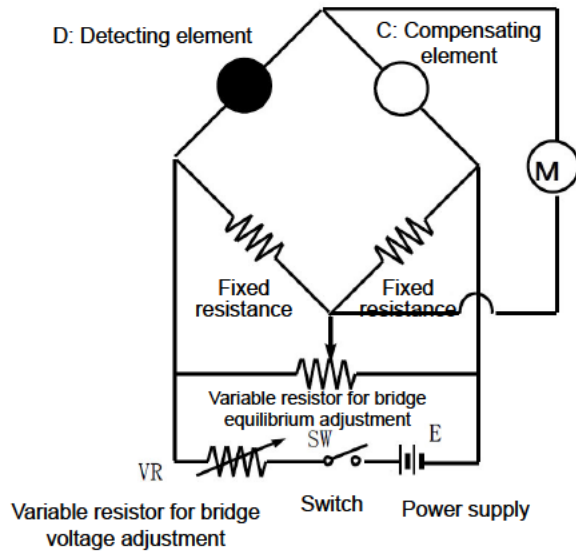
Basic Circuit
