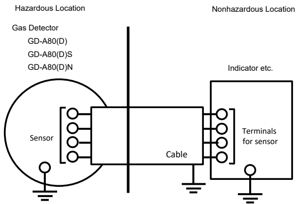
Installation Diagram
