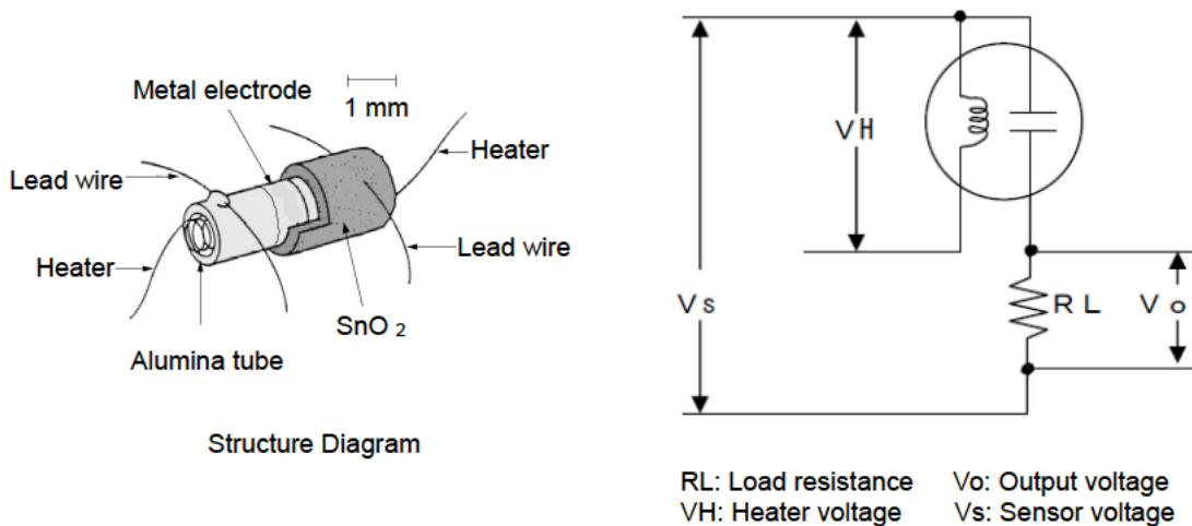
Basic Circuit
