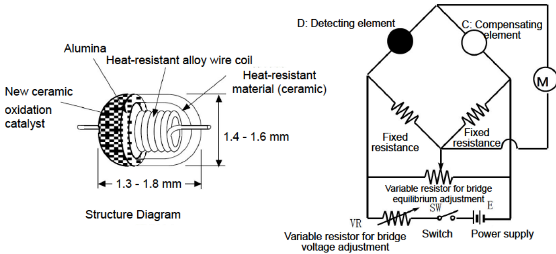
Basic Circuit
